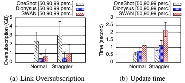
Figure 14: In WAN failure recovery, Dionysus significantly reduces oversubscription and update time as compared to SWAN. OneShot, while is fast, incurs huge oversubscription.
