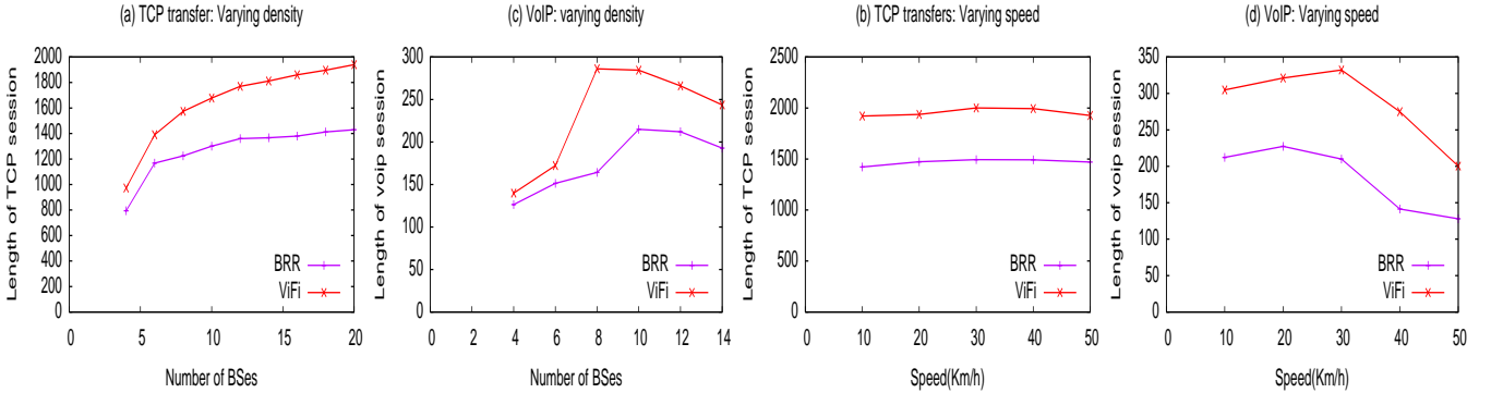
Figure 17: Comparisons between BRR and ViFi using the QualNet simulated environment for varying speed and density.
